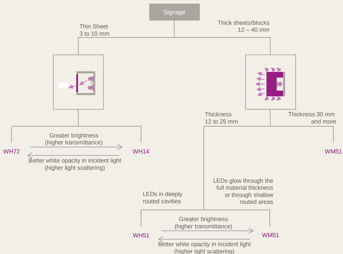
Fig. 4: Decision tree
