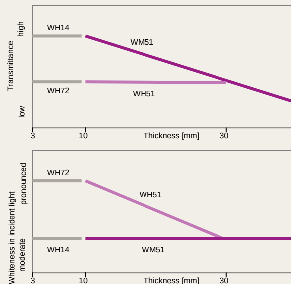
Fig. 1: Transmittance (top) and white opacity in incident light as a function of thickness.
